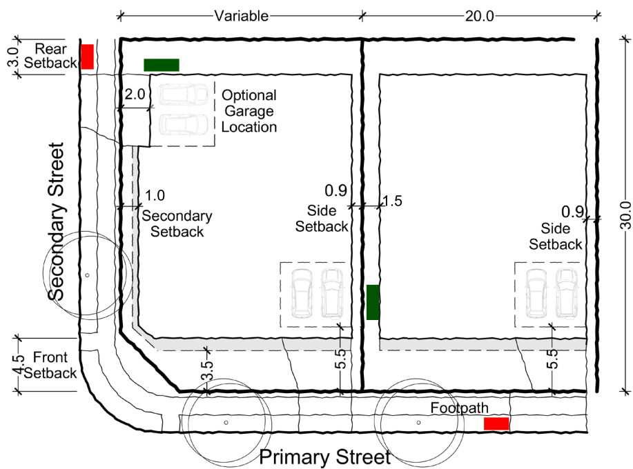
Example Built Form Typology Detached 20 x 30m (600sqm)
