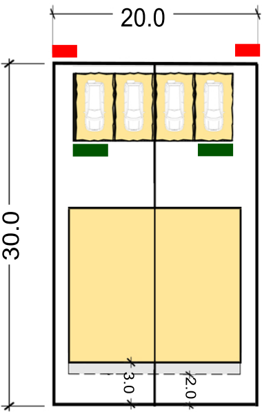
Typical Building Envelope Manor Home (Rear Loaded)
