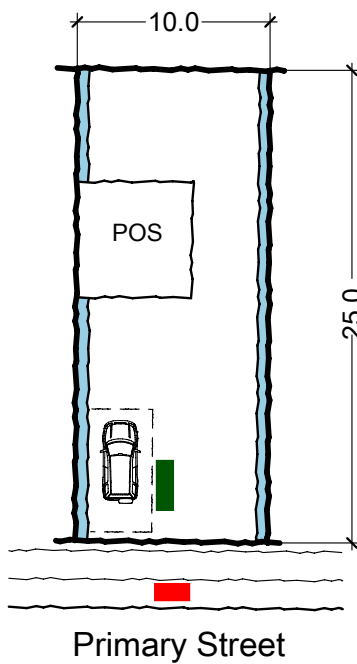
Typical Building Envelope Plan Live Work 10 x 25m (250sqm)
