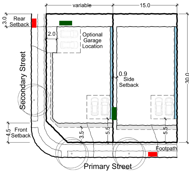
Typical Building Envelope Plan Detached 15 x 30m (450sqm)
