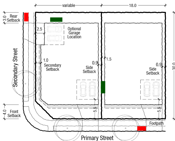
Typical Building Envelope Plan Detached 18 x 30m (540sqm)
