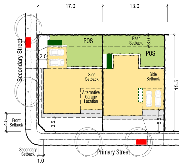
Typical Built Form Typology Patio Homes
