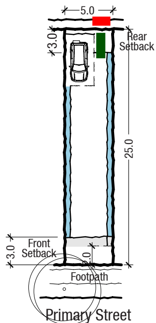
Typical Building Envelope Plan Attached 5 x 25m
