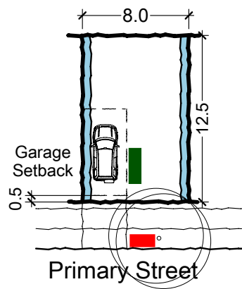
Typical Building Envelope Plan Urban Sleeve 8 x 12m (100sqm)
