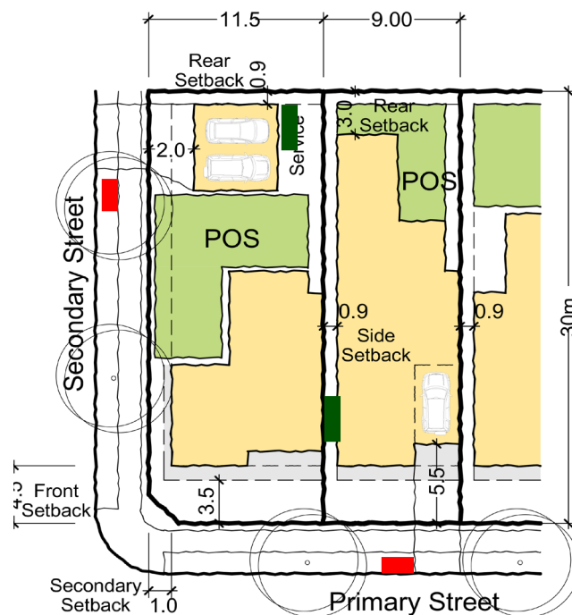
Example Built Form Typology Detached 11.5 x 30m (345sqm) Detached 9 x 30m (270sqm)
