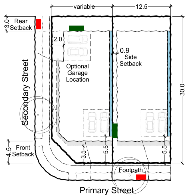
Typical Building Envelope Plan Detached 12.5 x 30m (375sqm)
