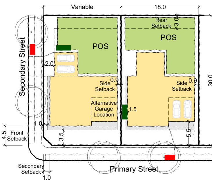
Typical Building Envelope Plan Detached 18 x 30m (540sqm)
