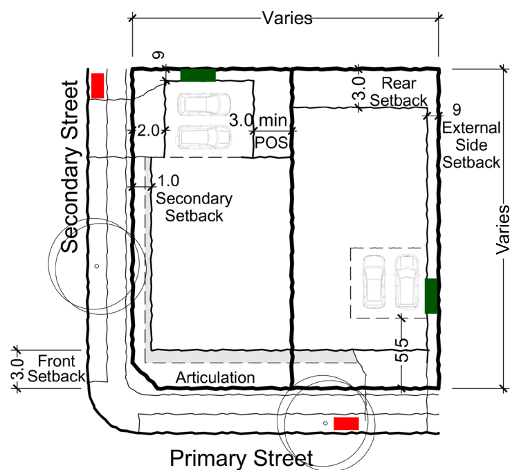
Typical Building Envelope Plan Corner Gallery
