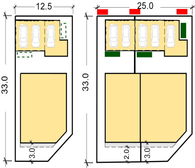
Typical Bulding Envelope Multi-Dwelling (Rear Loaded)
