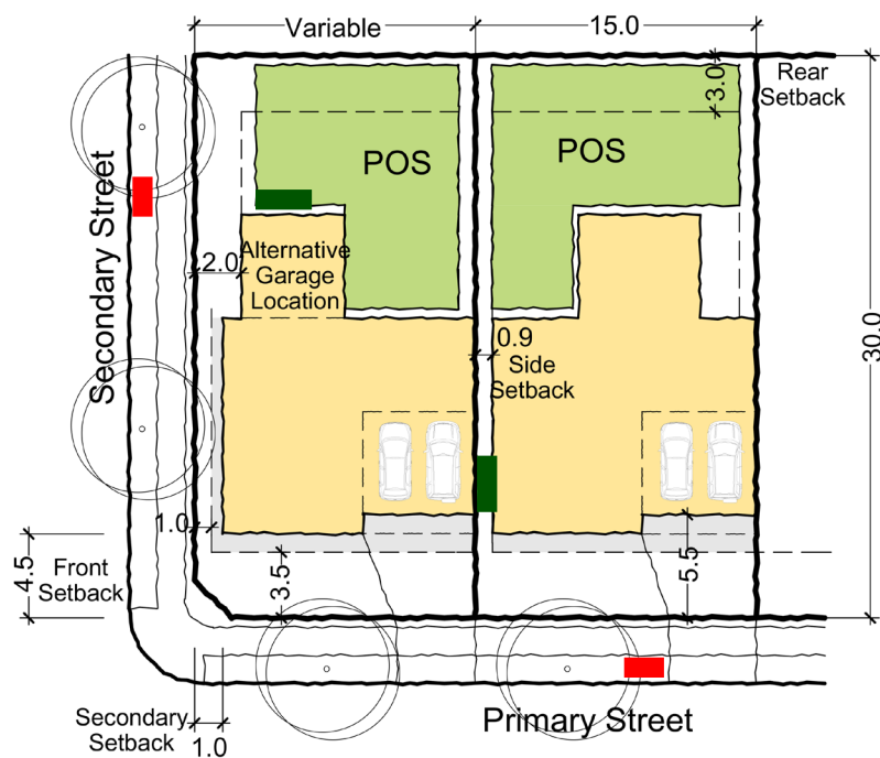
Example Built Form Typology Detached 15 x 30m (450sqm)
