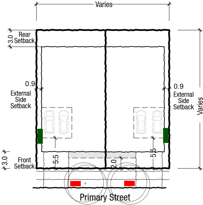
Typical Building Envelope Plan Gallery
