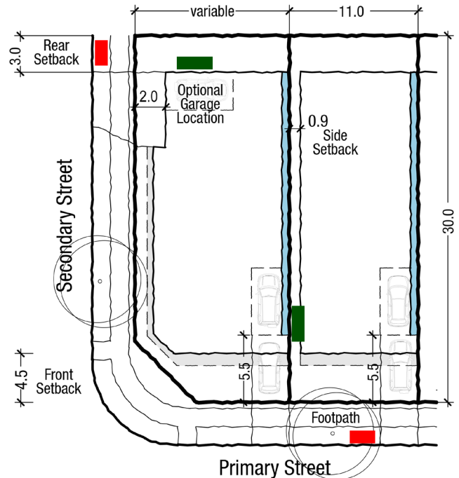
Typical Building Envelope Plan Detached 11 x 30m (330sqm)
