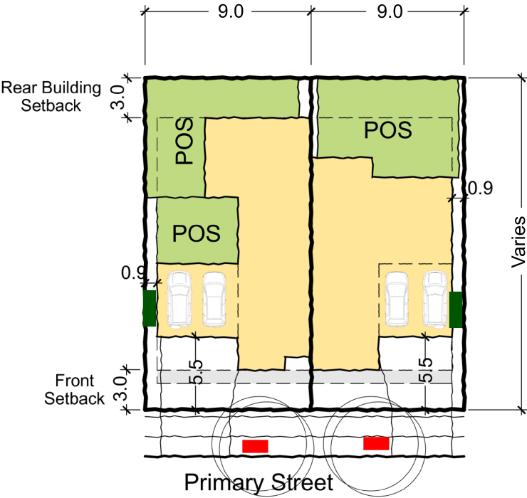
Example Built Form Typology Duplex
