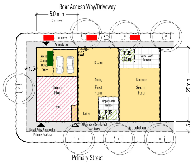
Typical Built Form Typology Shop Top
