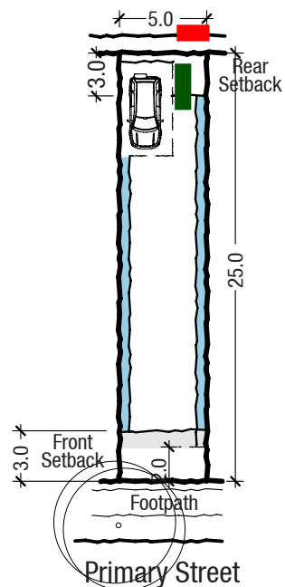
Typical Building Envelope Plan Attached 5 x 25m (125sqm)
