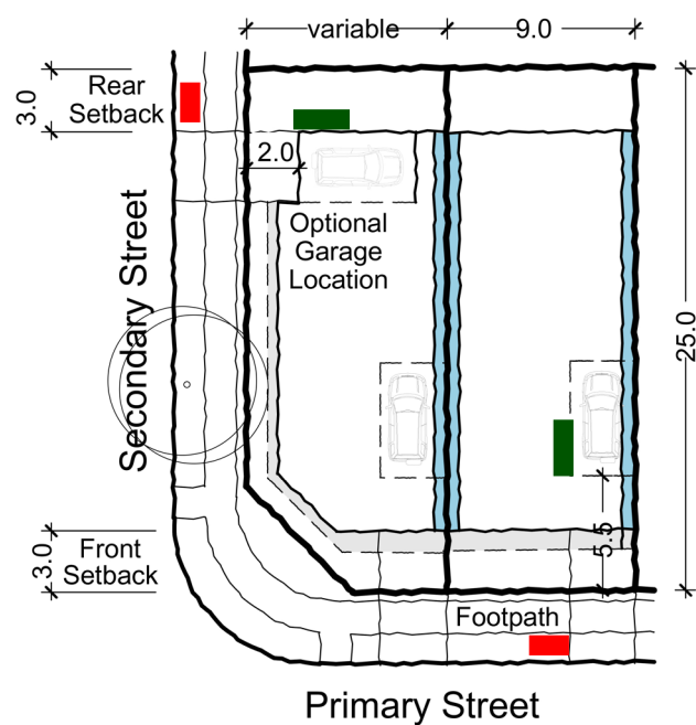
Typical Building Envelope Plan Attached 9 x 25m (225sqm)
