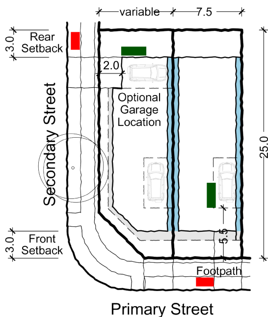
Typical Building Envelope Plan Attached 7.5 x 25m (187sqm)
