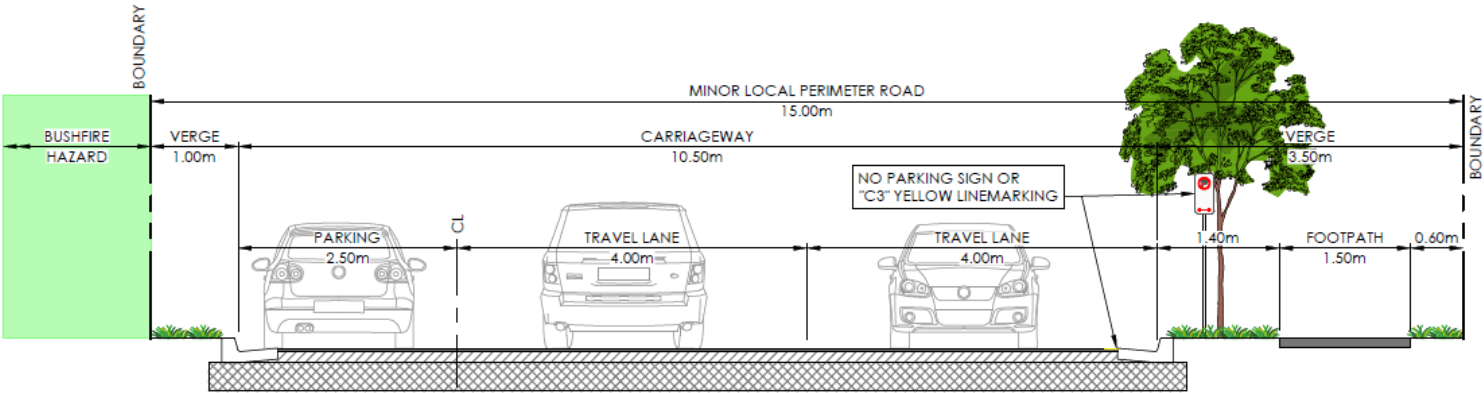
TYPICAL SECTION - MINOR LOCAL PERIMETER ROAD (ADJACENT TO BUSHFIRE HAZARD) OPTION B (1.0 - 10.5 - 3.5)
