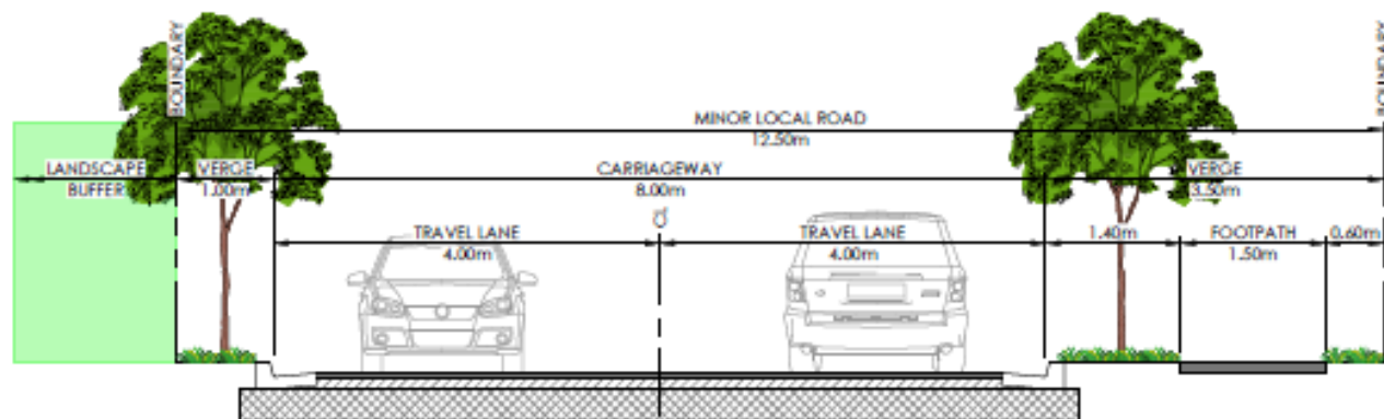
TYPICAL SECTION - MINOR LOCAL ROAD (THE NORTHERN ROAD INTERFACE) (1.0 - 8 - 3.5)
