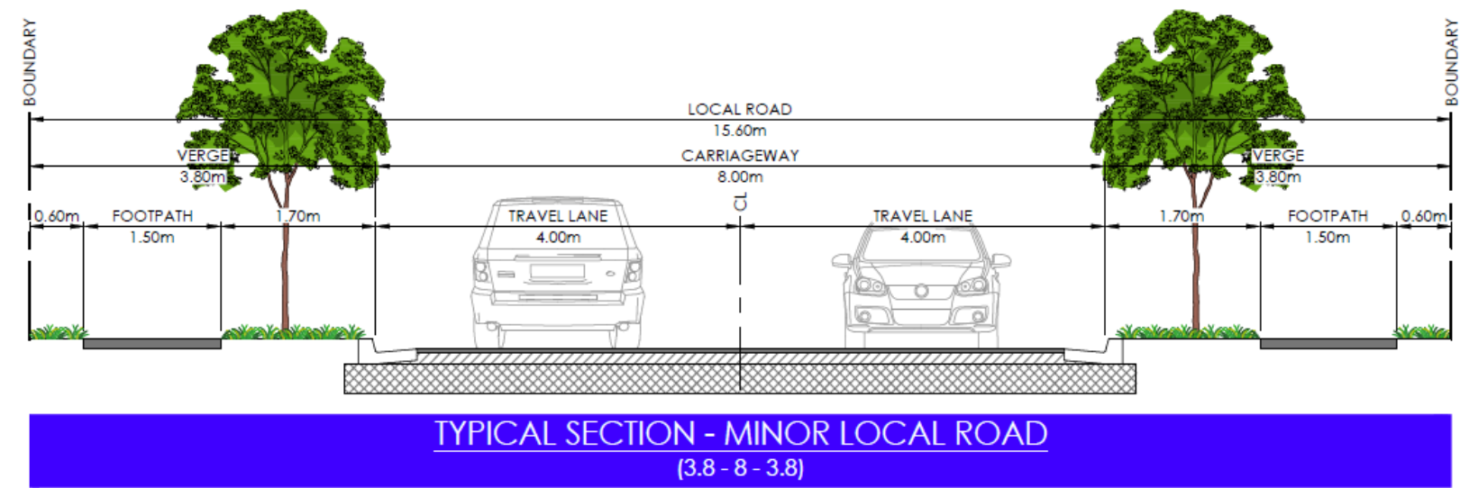
Figure E7.73 Minor Local Road
