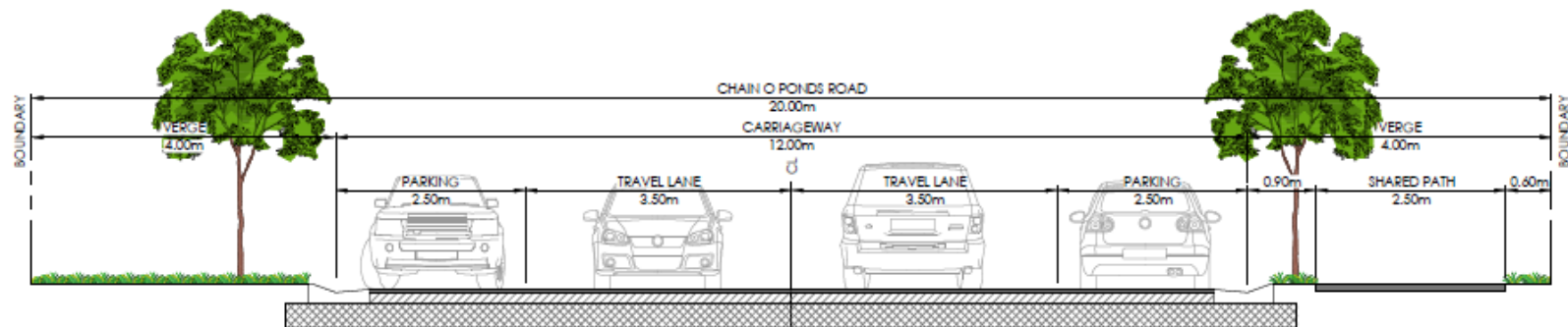
TYPICAL SECTION - CHAIN O PONDS ROAD (4.0 - 12 - 4.0)
