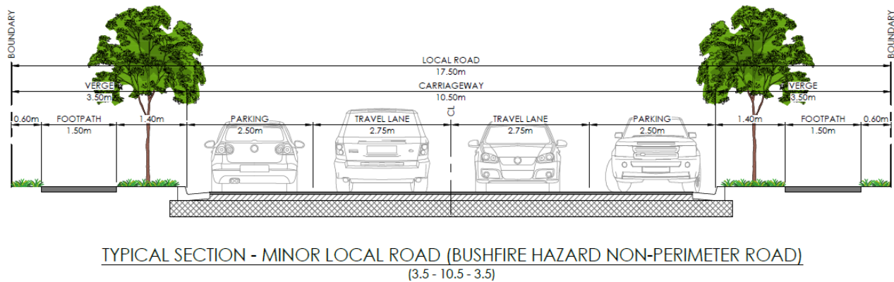
Figure E7.77 Minor Local Road (Bushfire Hazard Non-Perimeter Road)
