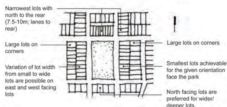
Figure E1.22 – Lot Design Principles
