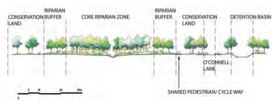
Figure E1.17 – Riparian Corridor (section)
